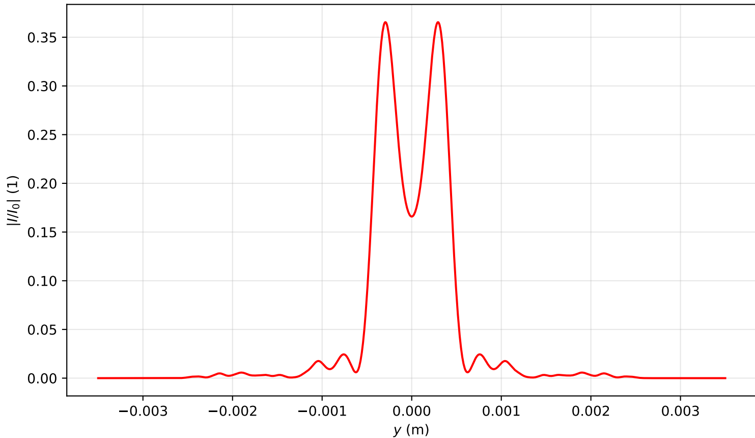
Intensity profile I(x=0, y, z=1.592)/I_0 , P_{in}=4.0P_{cr} , artificial time
